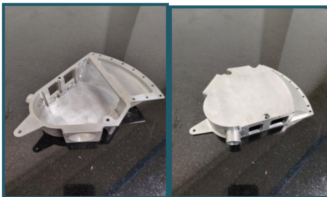
Compressor inlet plenum cover
